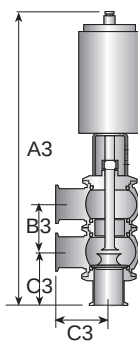
DIVERT-VALVE CLAMP & WELD
